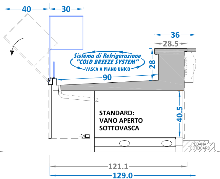
T-KOMPASS CBS 90 VD Vasca a piano unico
