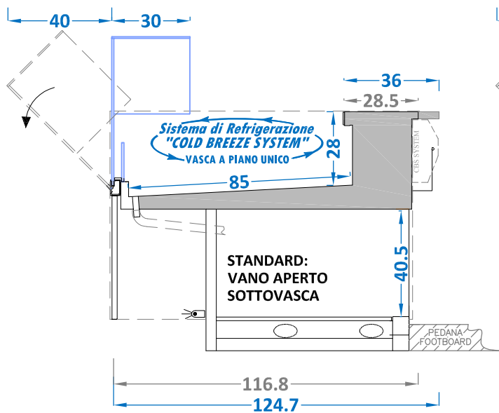
T-KOMPASS CBS 85 VD Vasca a piano unico
